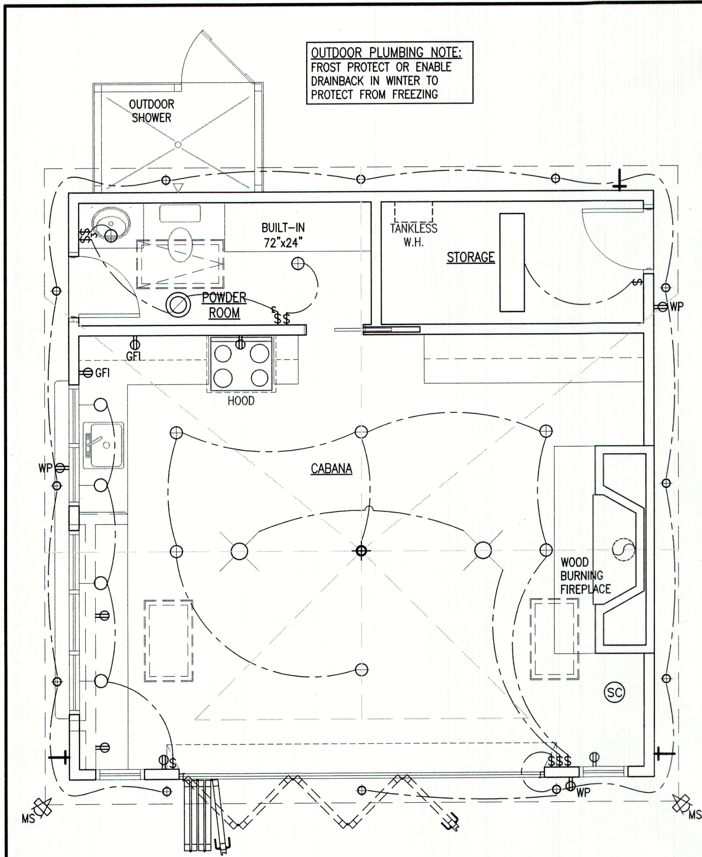
01 FIRST FLOOR PLAN (ELECTRICAL)
