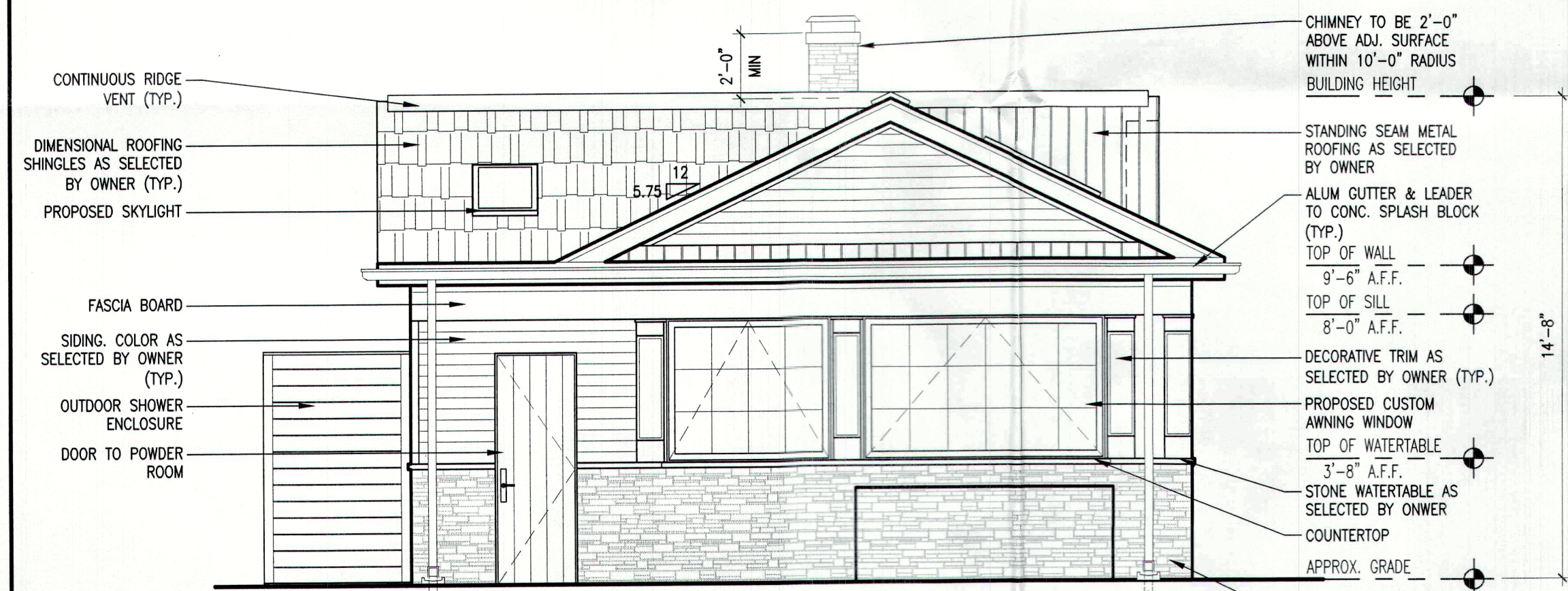
03 LEFT SIDE ELEVATION
