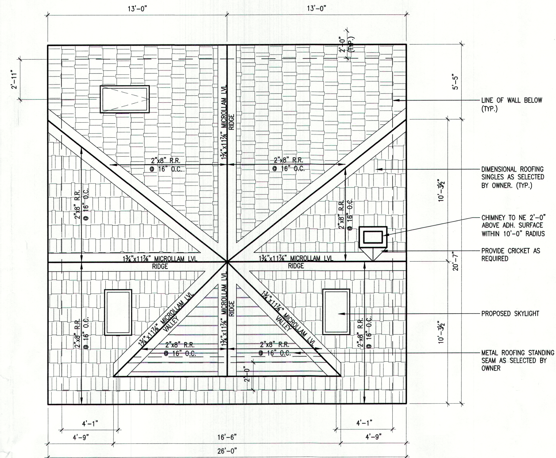
02 ROOF PLAN
