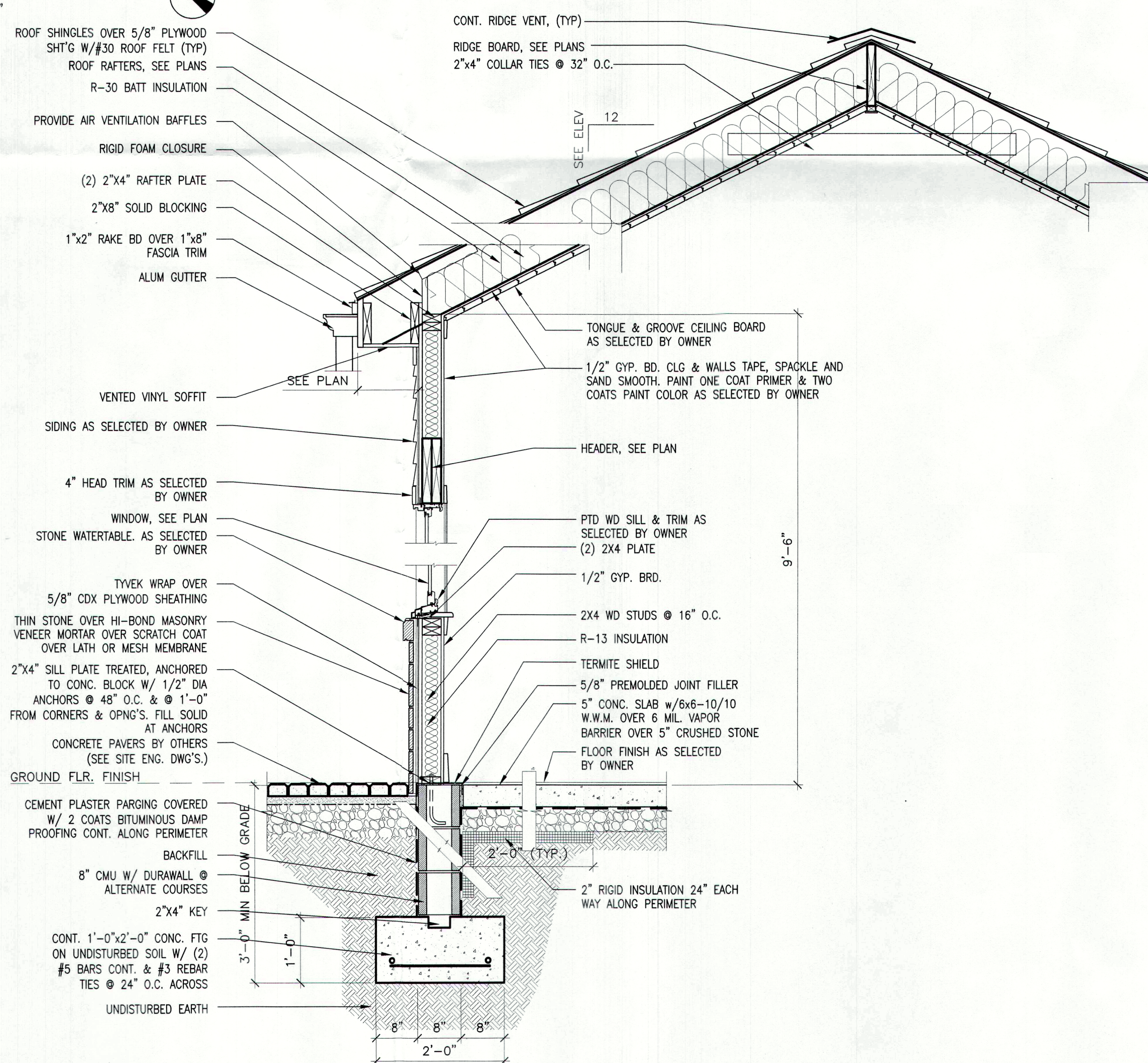
05 WALL SECTION
