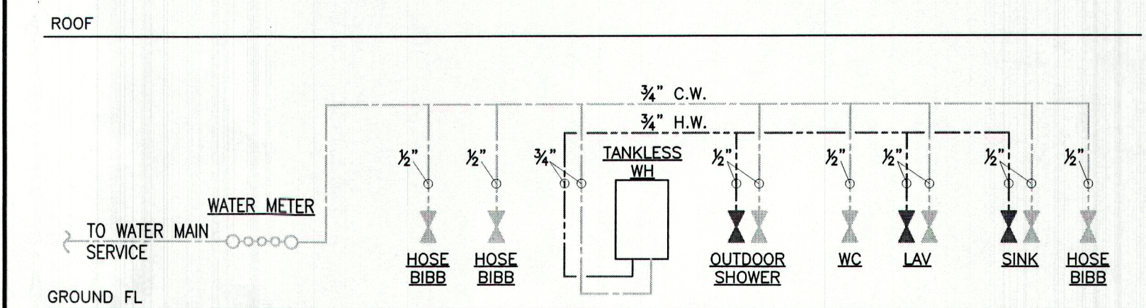
07 WATER SUPPLY RISER DIAGRAM
