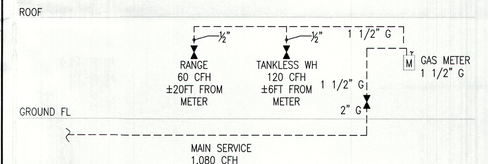
08 GAS SUPPLY RISER DIAGRAM
