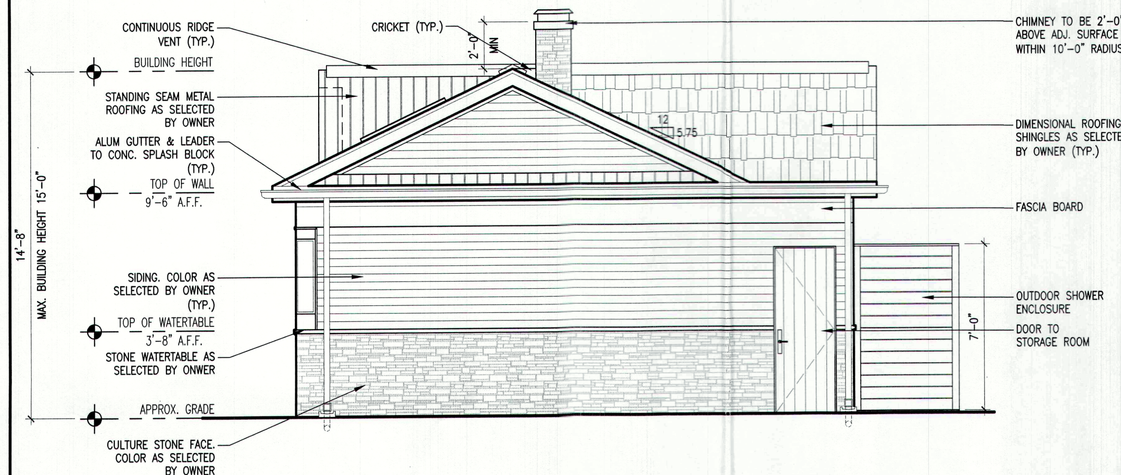
04 RIGHT SIDE ELEVATION
